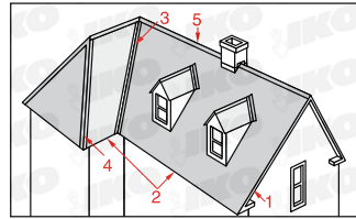
1. Rakes • 2. Eaves • 3. Valleys 4. Hips • 5. Ridges
