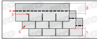
1. Exposure • 2. Headlap • 3. Cut-outs 4. Self Sealing Strip • 5. Tabs
